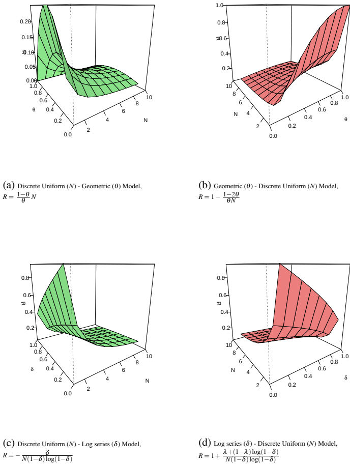
Figure 3: Plot of R for Discrete Uniform - Geometric, Geometric - Discrete Uniform and Discrete Uniform - Log series, Log series - Discrete Uniform models
