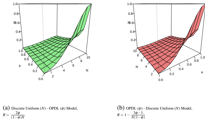
Figure 4: Plot of R for Discrete Uniform - OPDL and OPDL - Discrete Uniform model
